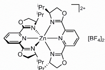
[2,6-Bis(( R )-4-isopropyl-4,5-dihydrooxazol-2-yl)pyridine]- [2,6-bis(( S )-4-isopropyl-4,5-dihydrooxazol-2-yl)pyridine]zinc(II) ditetrafluoroborate C_{34}H_{46}B_2F_8N_6O_4Zn Compound ( RS )-2
