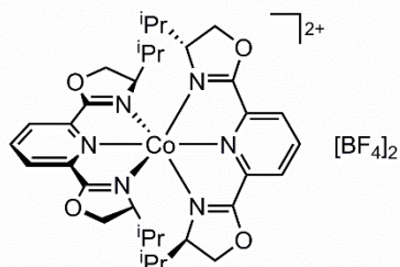
Bis[2,6-bis(( R )-4-isopropyl-4,5-dihydrooxazol-2-yl)pyridine]cobalt(II) ditetrafluoroborate C_{34}H_{46}B_2CoF_8N_6O_4 Compound ( R )-4
