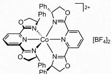
Bis[2,6-bis(( R )-4-phenyl-4,5-dihydrooxazol-2-yl)pyridine]cobalt(II) ditetrafluoroborate C_{46}H_{38}B_2CoF_8N_6O_4 Compound ( R )-3
