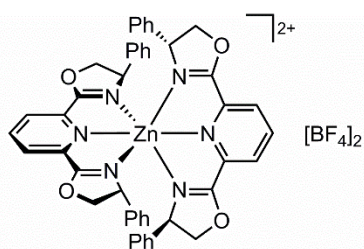
Bis[2,6-bis(( R )-4-phenyl-4,5-dihydrooxazol-2-yl)pyridine]zinc(II) ditetrafluoroborate C_{46}H_{38}B_2F_8N_6O_4Zn Compound ( R )-1
