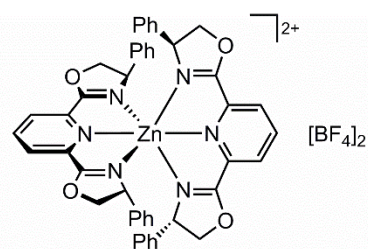
[2,6-Bis(( R )-4-phenyl-4,5-dihydrooxazol-2-yl)pyridine]- [2,6-bis(( S )-4-phenyl-4,5-dihydrooxazol-2-yl)pyridine]zinc(II) ditetrafluoroborate C_{46}H_{38}B_2F_8N_6O_4Zn Compound ( RS )-1
