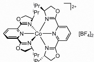
[2,6-Bis(( R )-4-isopropyl-4,5-dihydrooxazol-2-yl)pyridine]- [2,6-bis(( S )-4-isopropyl-4,5-dihydrooxazol-2-yl)pyridine]cobalt(II) ditetrafluoroborate C_{34}H_{46}B_2CoF_8N_6O_4 Compound ( RS )-4
