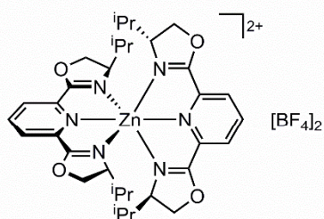
Bis[2,6-bis(( R )-4-isopropyl-4,5-dihydrooxazol-2-yl)pyridine]zinc(II) ditetrafluoroborate C_{34}H_{46}B_2F_8N_6O_4Zn Compound ( R )-2
