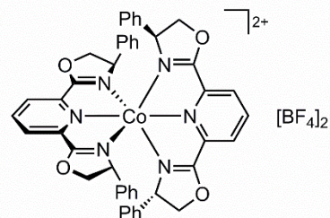
[2,6-Bis(( R )-4-phenyl-4,5-dihydrooxazol-2-yl)pyridine]- [2,6-bis(( S )-4-phenyl-4,5-dihydrooxazol-2-yl)pyridine]cobalt(II) ditetrafluoroborate C_{46}H_{38}B_2CoF_8N_6O_4 Compound ( RS )-3
