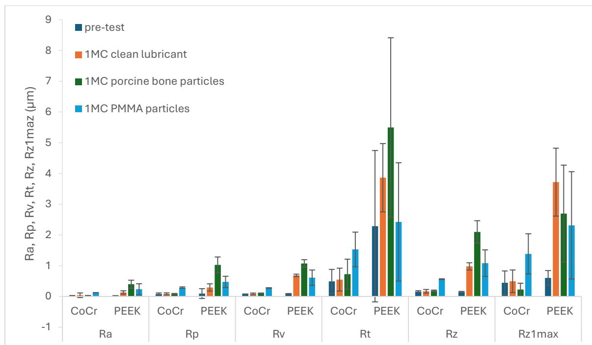
Supplementary Figure 3: Mean Ra, Rp, Rv, Rt, Rz and Rz1max (μm) ± 95% CL of femoral components articulating against PEEK and CoCr femoral components at each measurement point, N=3.
