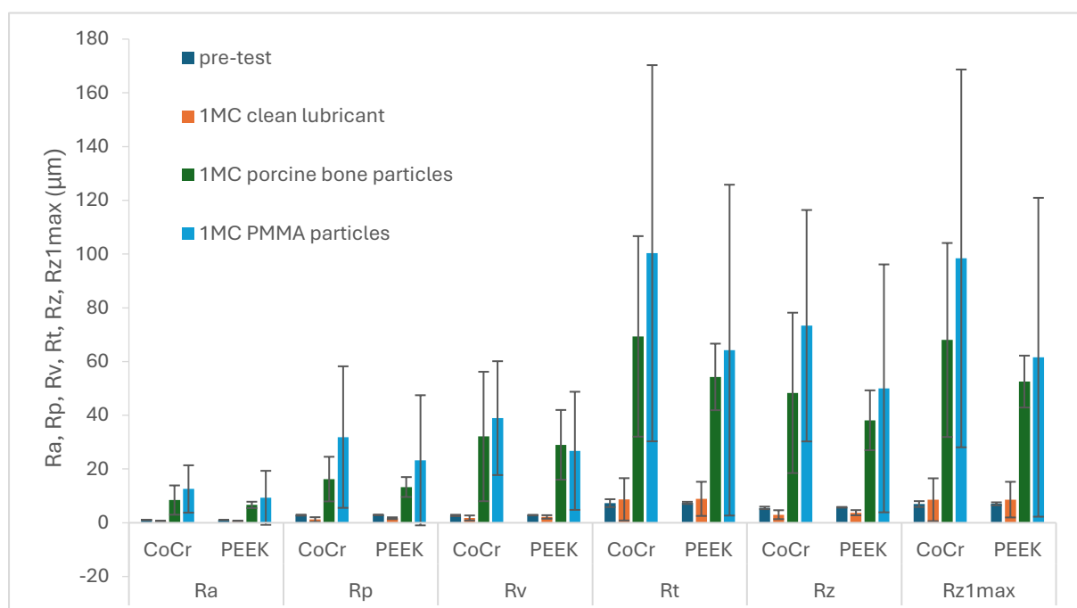
Supplementary Figure 2: Mean Ra, Rp, Rv, Rt, Rz and Rz1max (μm) ± 95% CL of tibial components articulating against PEEK and CoCr femoral components at each measurement point, N=3.
