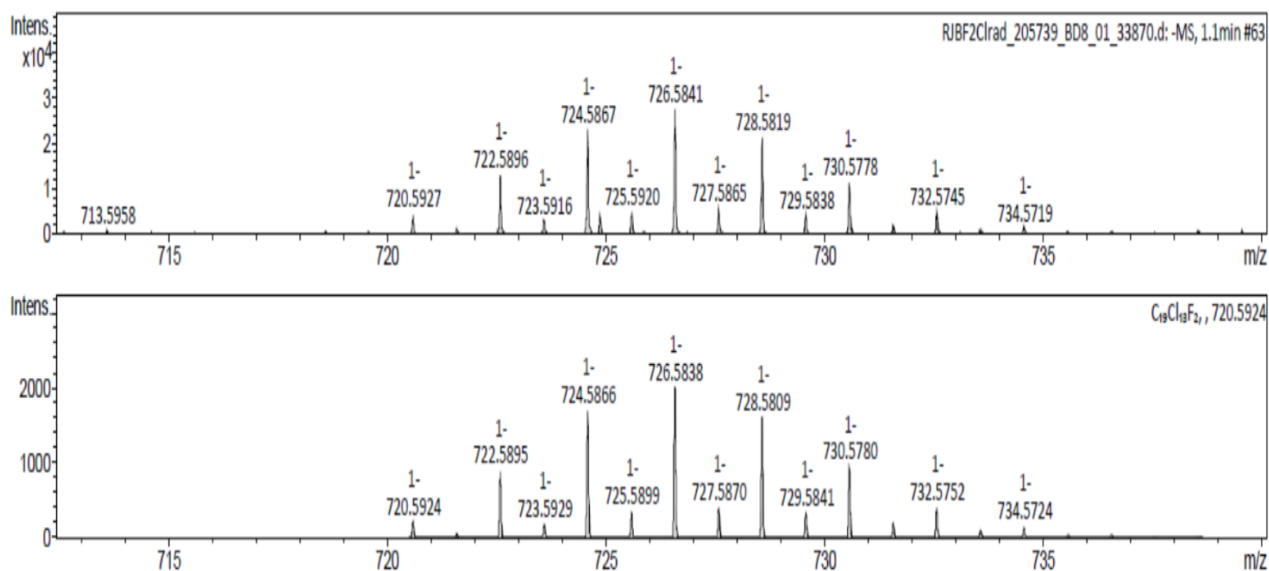
Radical 10b (above) MS parent ion ( M^\bullet ). (below) simulated for C_{19}Cl_{13}F_2^\bullet
