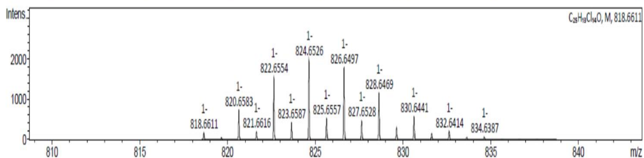
Radical 7a (above) MS parent ion ( M^- ). (below) simulated for C_{19}Cl_{14}(OHx)^-
