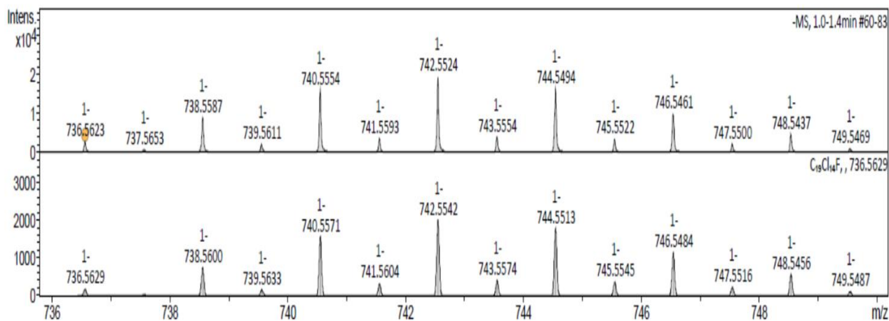
Radical 10a (above) MS parent ion ( M^\bullet ). (below) simulated for C_{19}Cl_{14}F^\bullet
